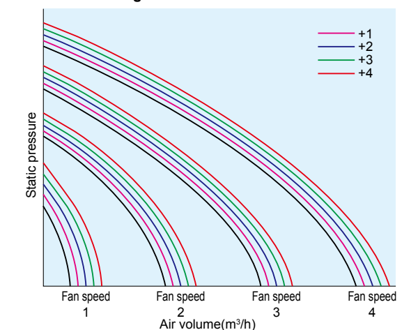
■ P-Q curve image
