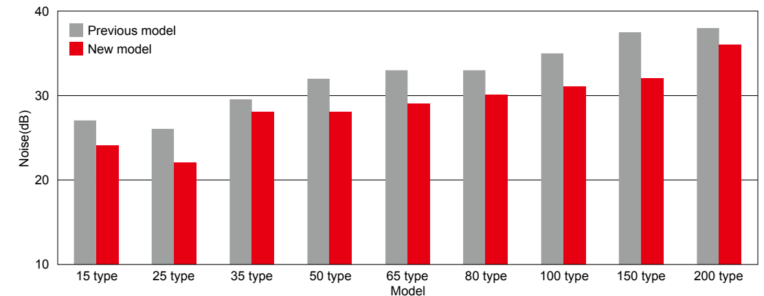
■ Noise comparison between new and previous models (new model: fanspeed3, previous model: High)
